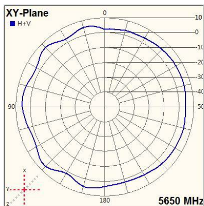
Signal Coverage Pattern for 5GHz
